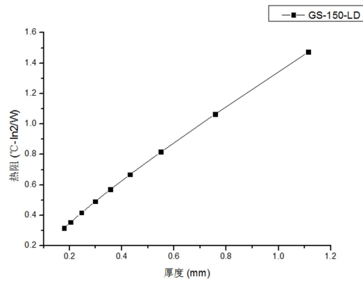
GS-150-LD Thickness vs Thermal Resistance
